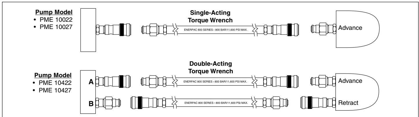
Figure 4, Coupling Diagram
