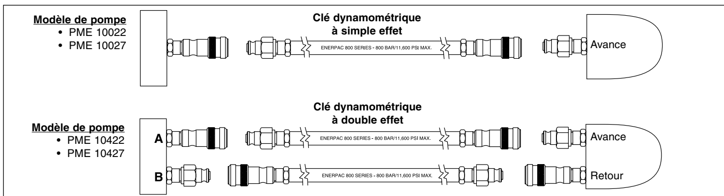
Figure 4, Schéma des raccords
